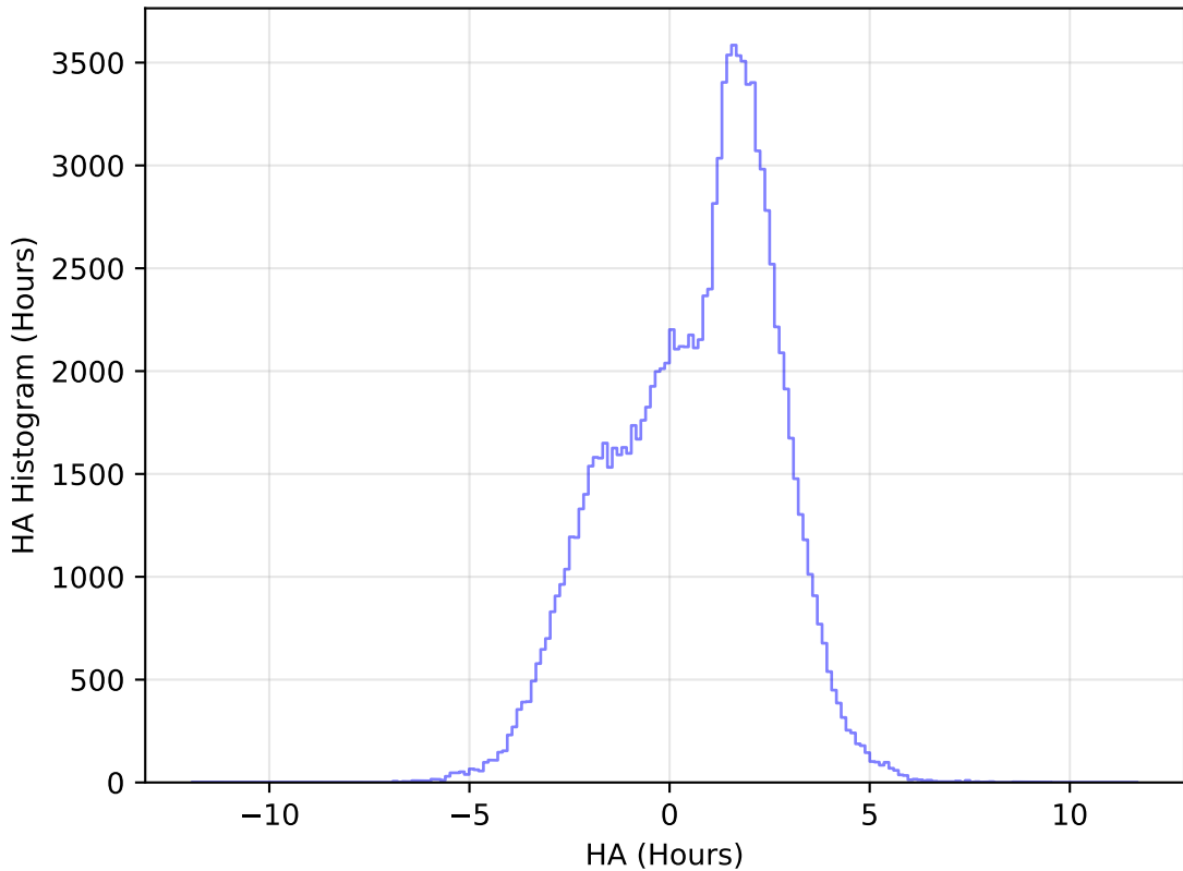
ddf_loaded_half_fl8_v3.4_10yrs All sky u band: HA Histogram
