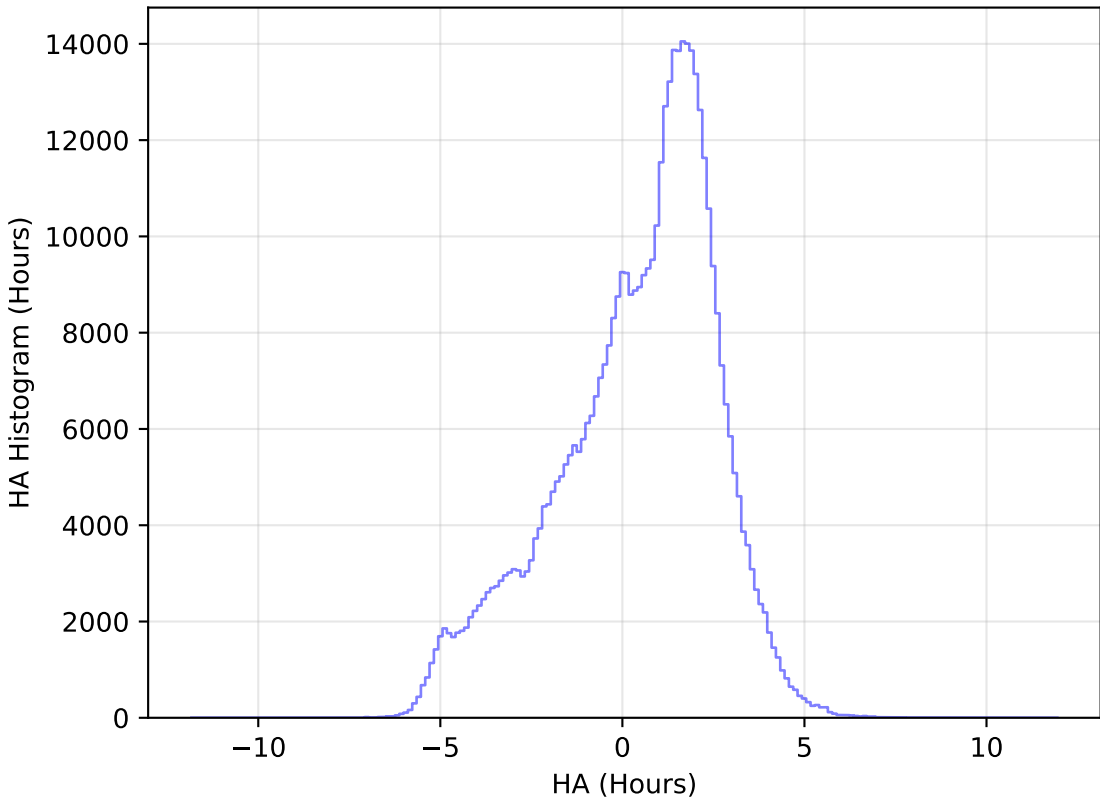
ddf_loaded_half_fl8_v3.4_10yrs All sky r band: HA Histogram
