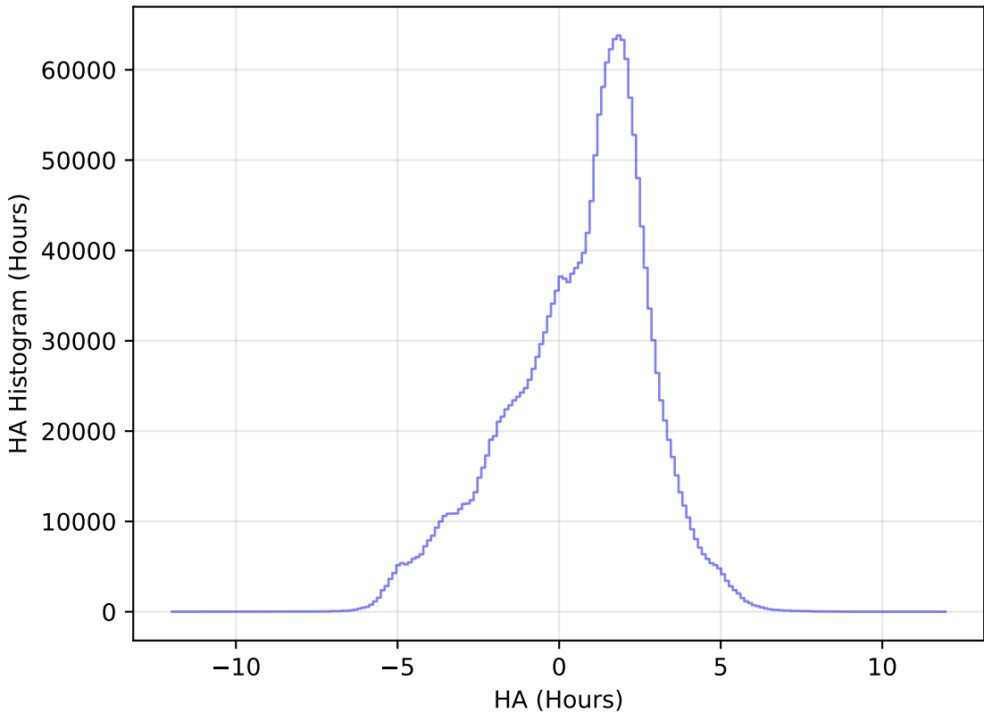
ddf_loaded_half_fl8_v3.4_10yrs All sky all bands: HA Histogram
