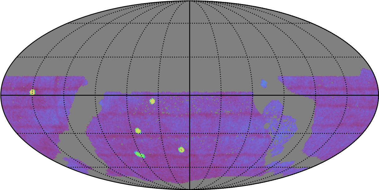
ddf_loaded_half_fl8_v3.4_10yrs gri WFD: Fraction of visits with a revisit < 60 min
