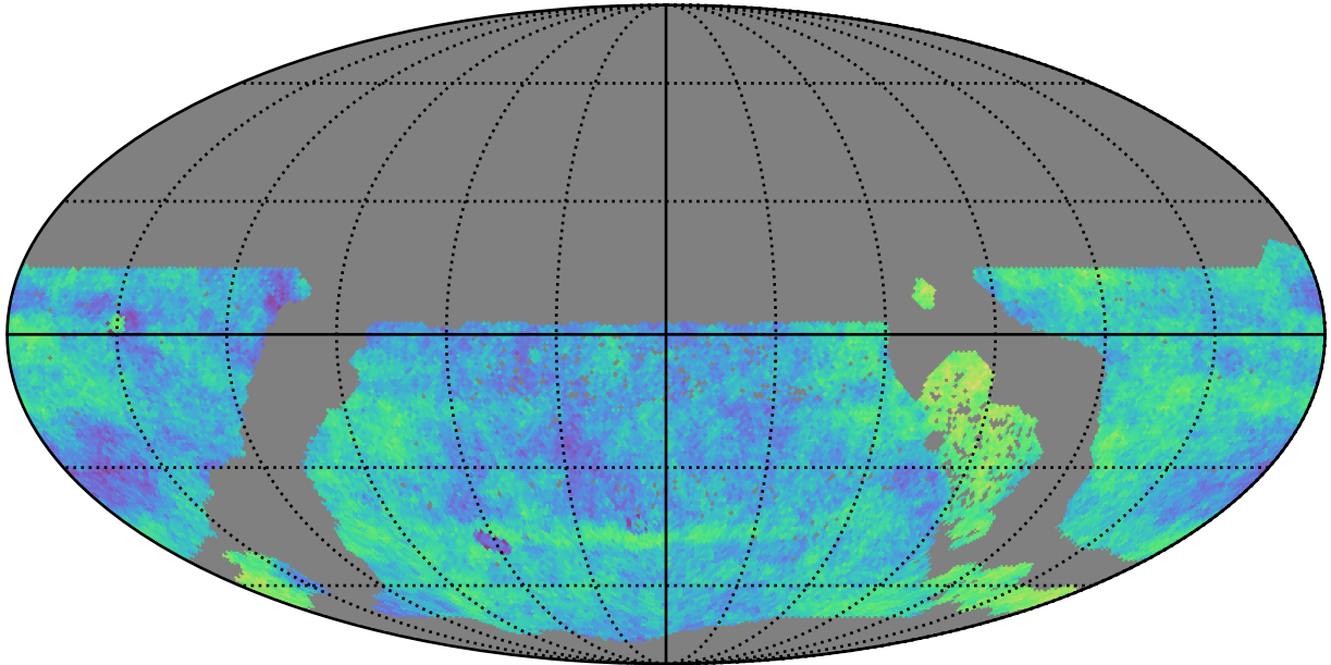
ddf_loaded_half_fl8_v3.4_10yrs gri WFD: Fraction of visits in pairs (20-90 min)
