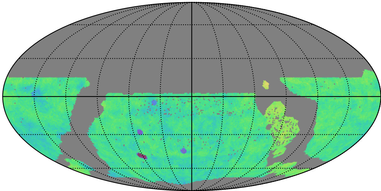
ddf_loaded_half_fl8_v3.4_10yrs gri WFD: Fraction of visits in pairs (10-60 min)
