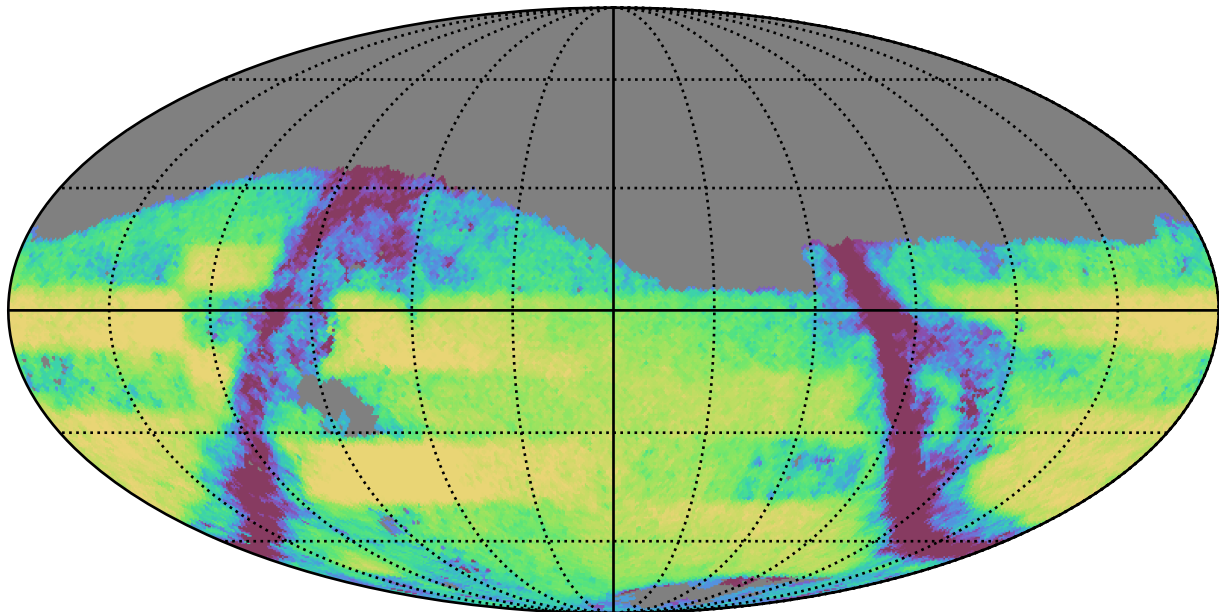
ddf_loaded_half_fl8_v3.4_10yrs Yr 3-4 r band: Exgal_CoaddM5
