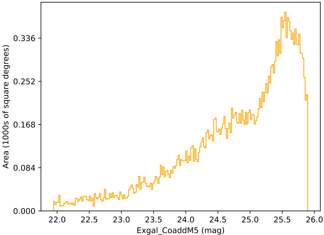
ddf_loaded_half_fl8_v3.4_10yrs Yr 3-4 r band: Exgal_CoaddM5
