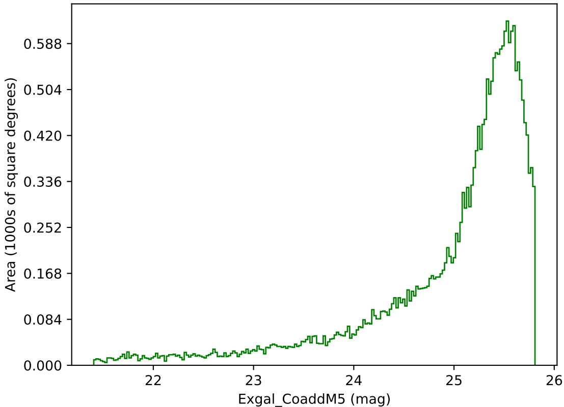
ddf_loaded_half_fl8_v3.4_10yrs Yr 1 g band: Exgal_CoaddM5
