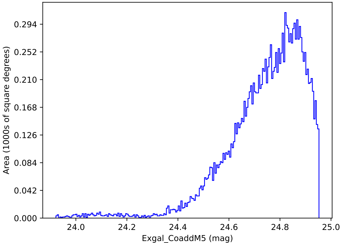
ddf_loaded_half_fl8_v3.4_10yrs WFD y band: Exgal_CoaddM5
