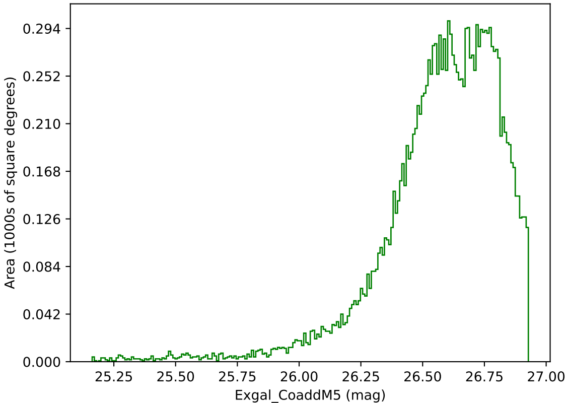
ddf_loaded_half_fl8_v3.4_10yrs WFD g band: Exgal_CoaddM5
