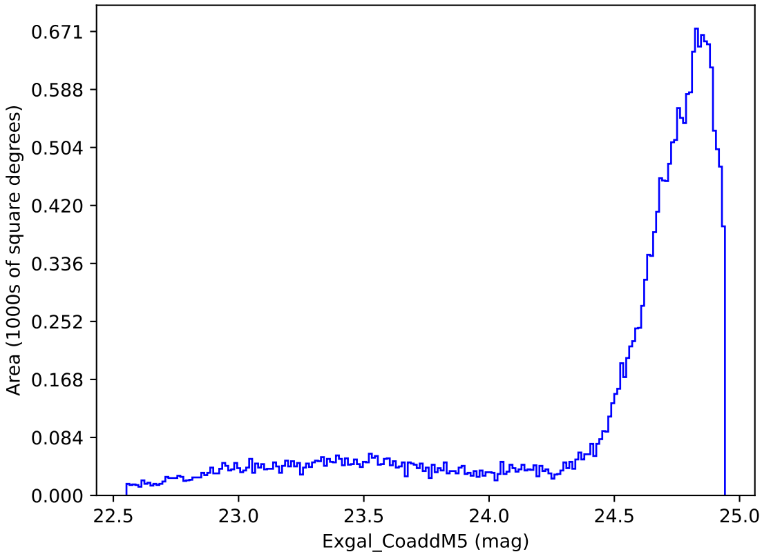
ddf_loaded_half_fl8_v3.4_10yrs All sky y band: Exgal_CoaddM5
