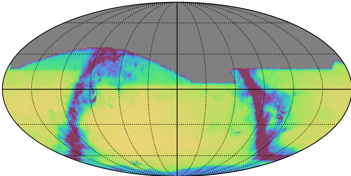
ddf_loaded_half_fl8_v3.4_10yrs All sky r band: Exgal_CoaddM5
