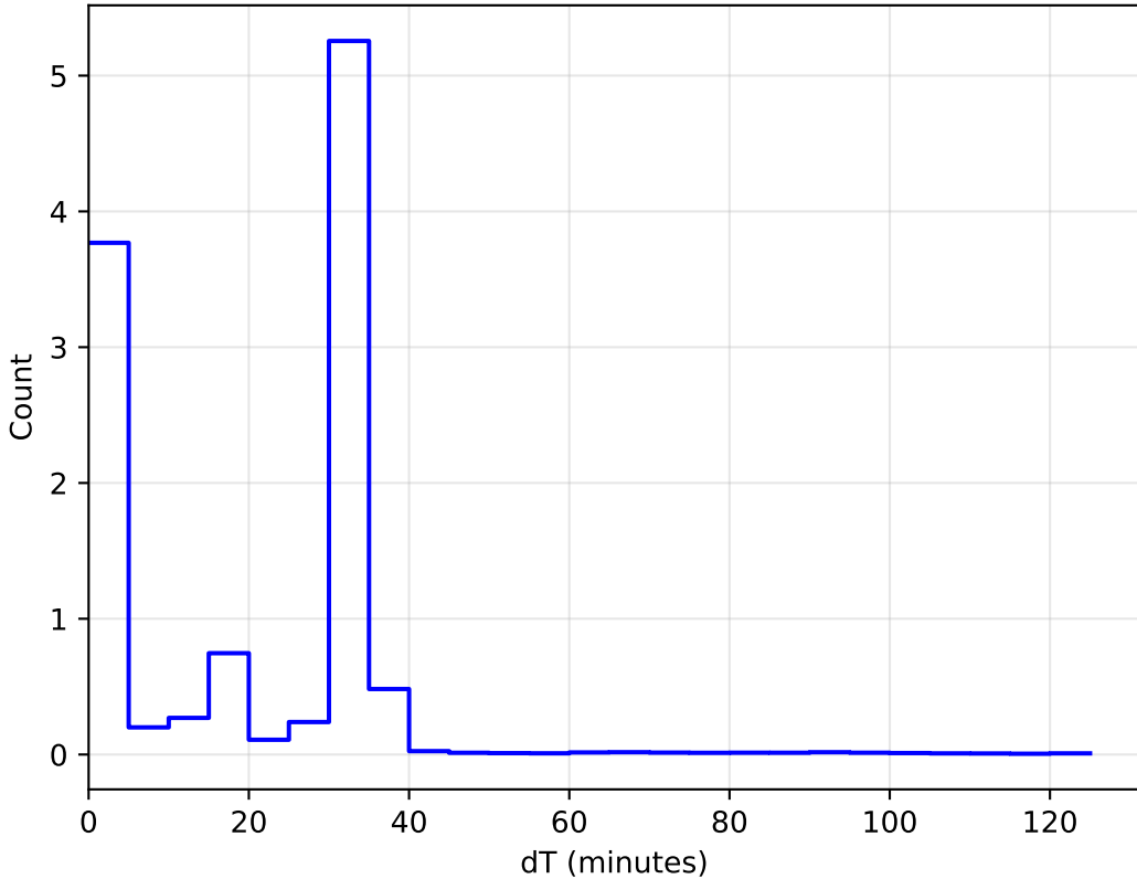
ddf_loaded_half_fl8_v3.4_10yrs WFD: DeltaT Histogram
