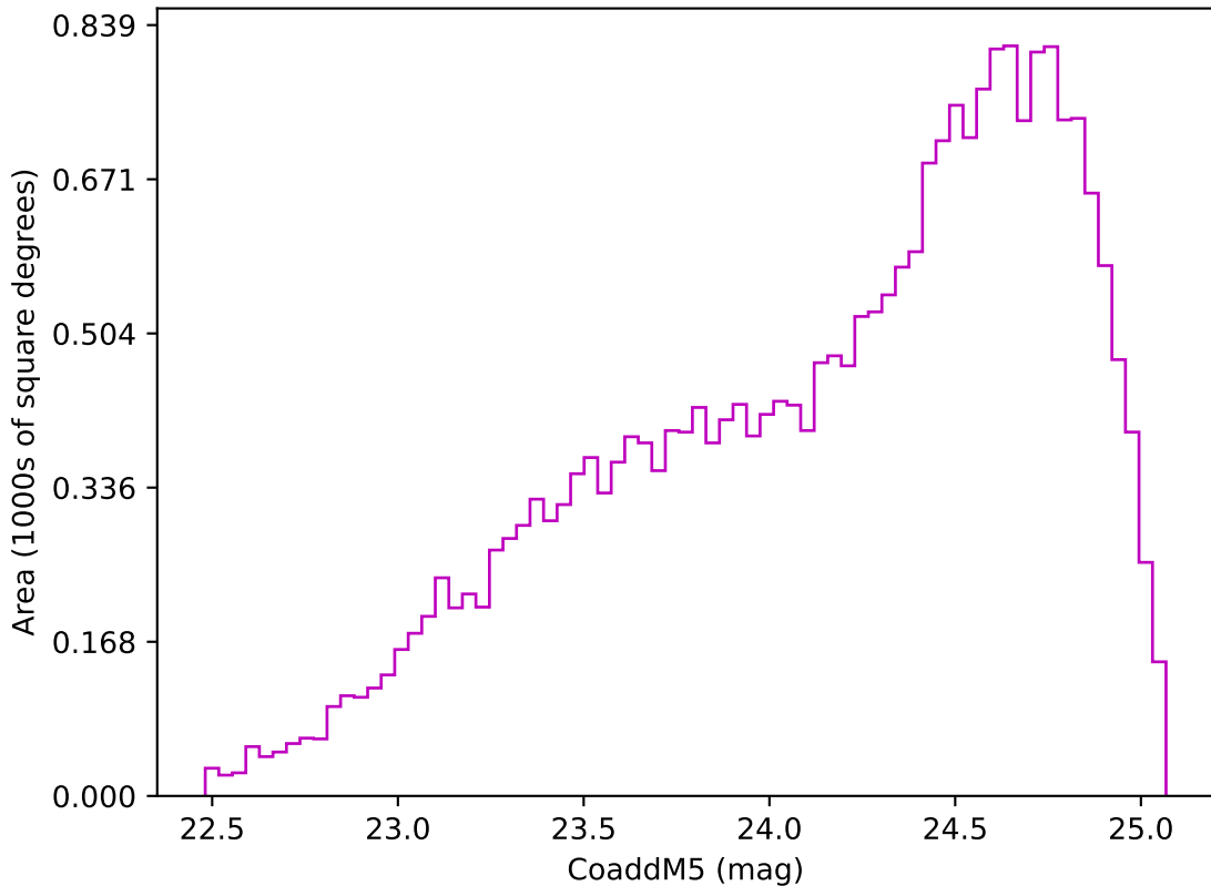
ddf_loaded_half_fl8_v3.4_10yrs Yr 3-4 z band: CoaddM5
