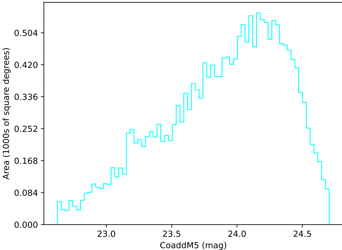
ddf_loaded_half_fl8_v3.4_10yrs Yr 3-4 u band: CoaddM5
