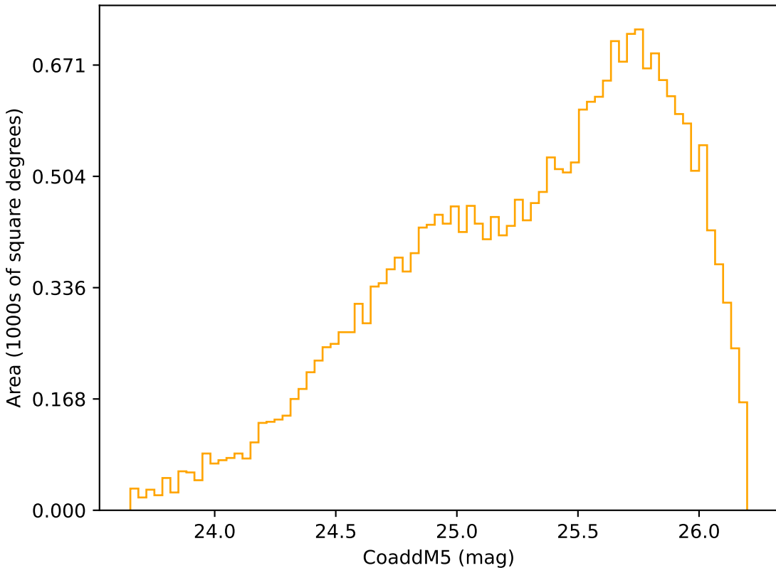
ddf_loaded_half_fl8_v3.4_10yrs Yr 3-4 r band: CoaddM5
