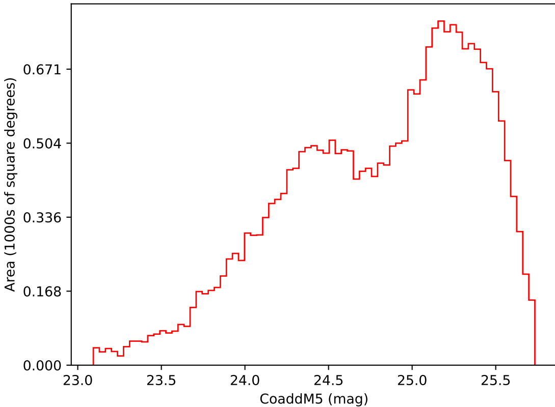
ddf_loaded_half_fl8_v3.4_10yrs Yr 3-4 i band: CoaddM5
