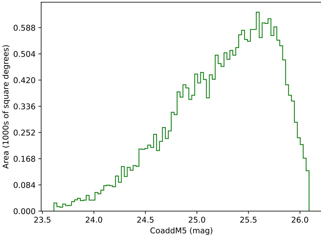
ddf_loaded_half_fl8_v3.4_10yrs Yr 3-4 g band: CoaddM5
