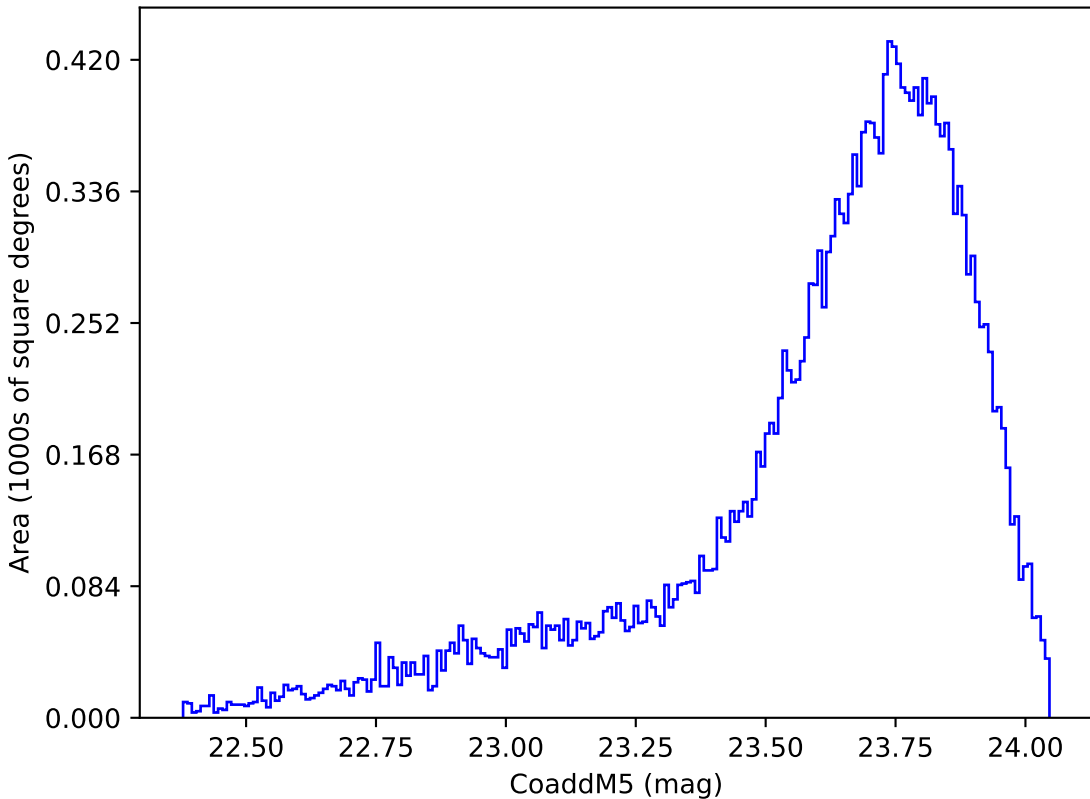
ddf_loaded_half_f18_v3.4_10yrs Yr 1 y band: CoaddM5
