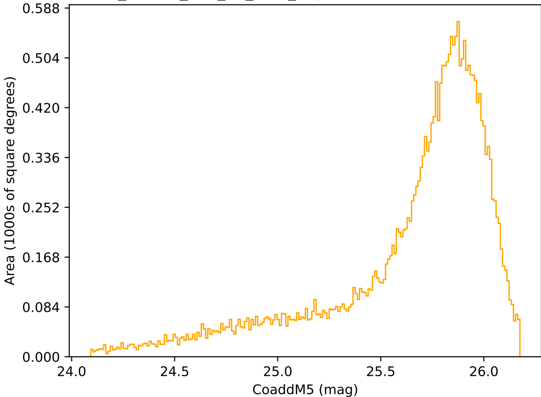
ddf_loaded_half_fl8_v3.4_10yrs Yr 1 r band: CoaddM5
