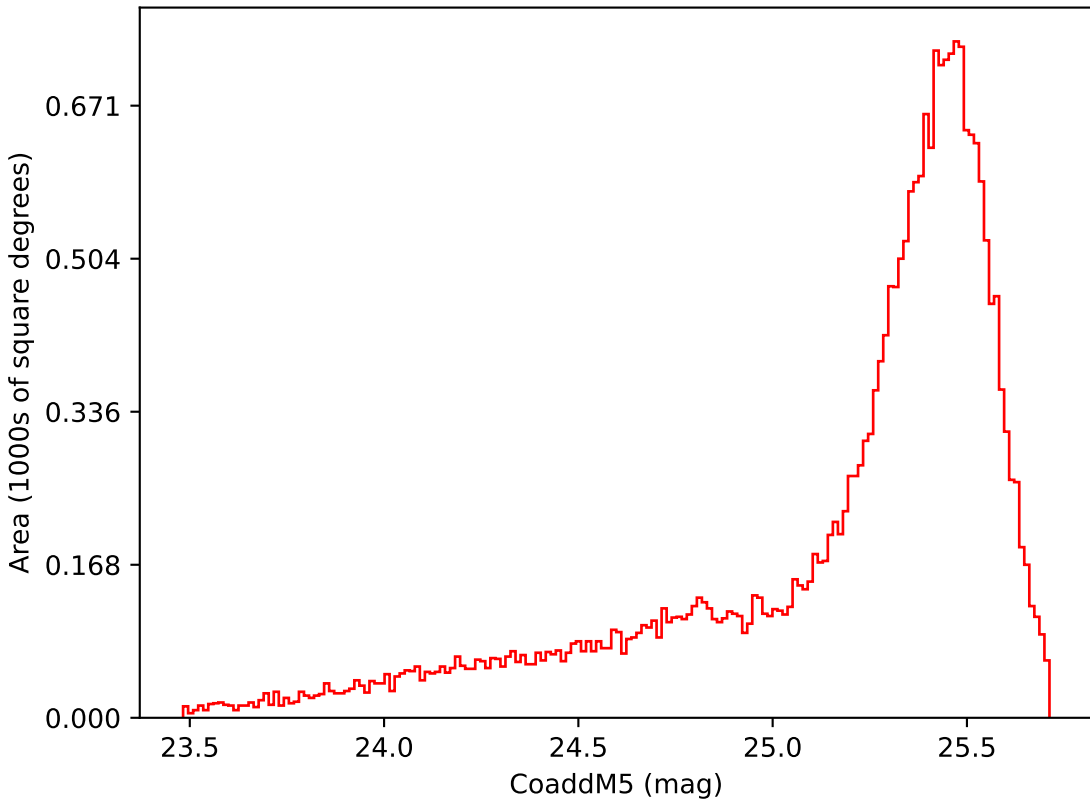
ddf_loaded_half_fl8_v3.4_10yrs Yr 1 i band: CoaddM5
