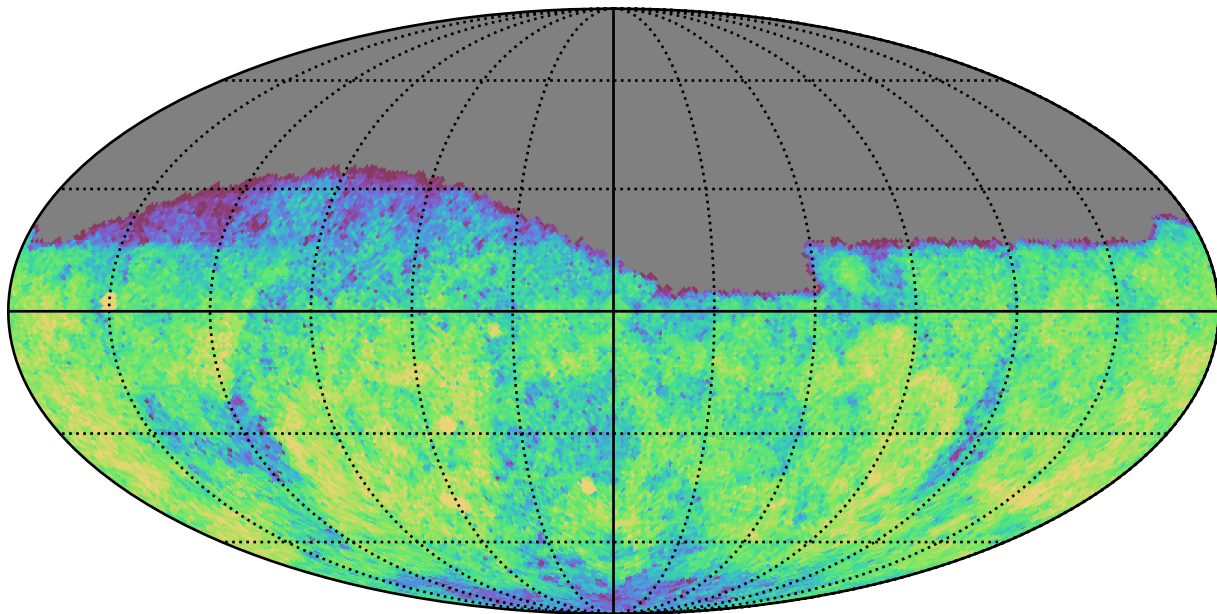
ddf_loaded_half_fl8_v3.4_10yrs Yr 1 g band: CoaddM5
