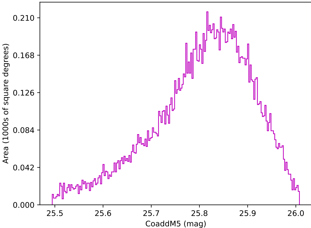
ddf_loaded_half_fl8_v3.4_10yrs WFD z band: CoaddM5
