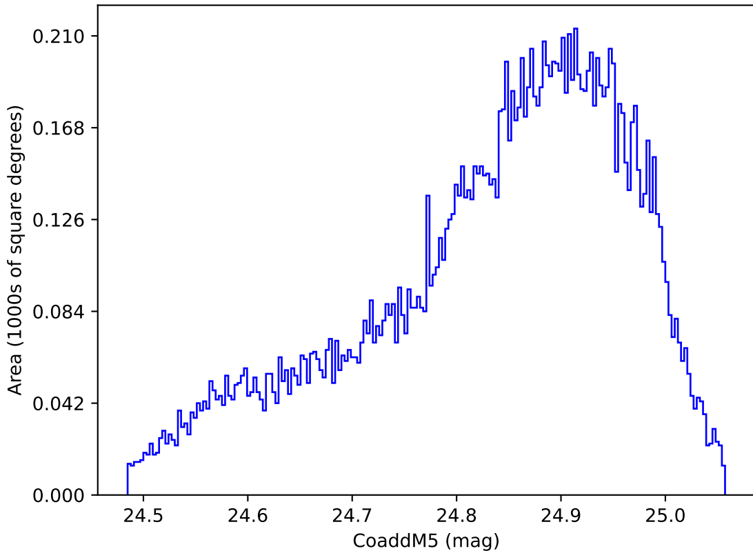
ddf_loaded_half_fl8_v3.4_10yrs WFD y band: CoaddM5
