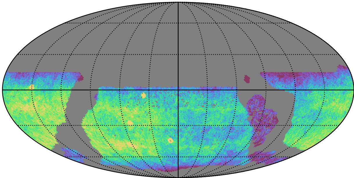
ddf_loaded_half_fl8_v3.4_10yrs WFD u band: CoaddM5
