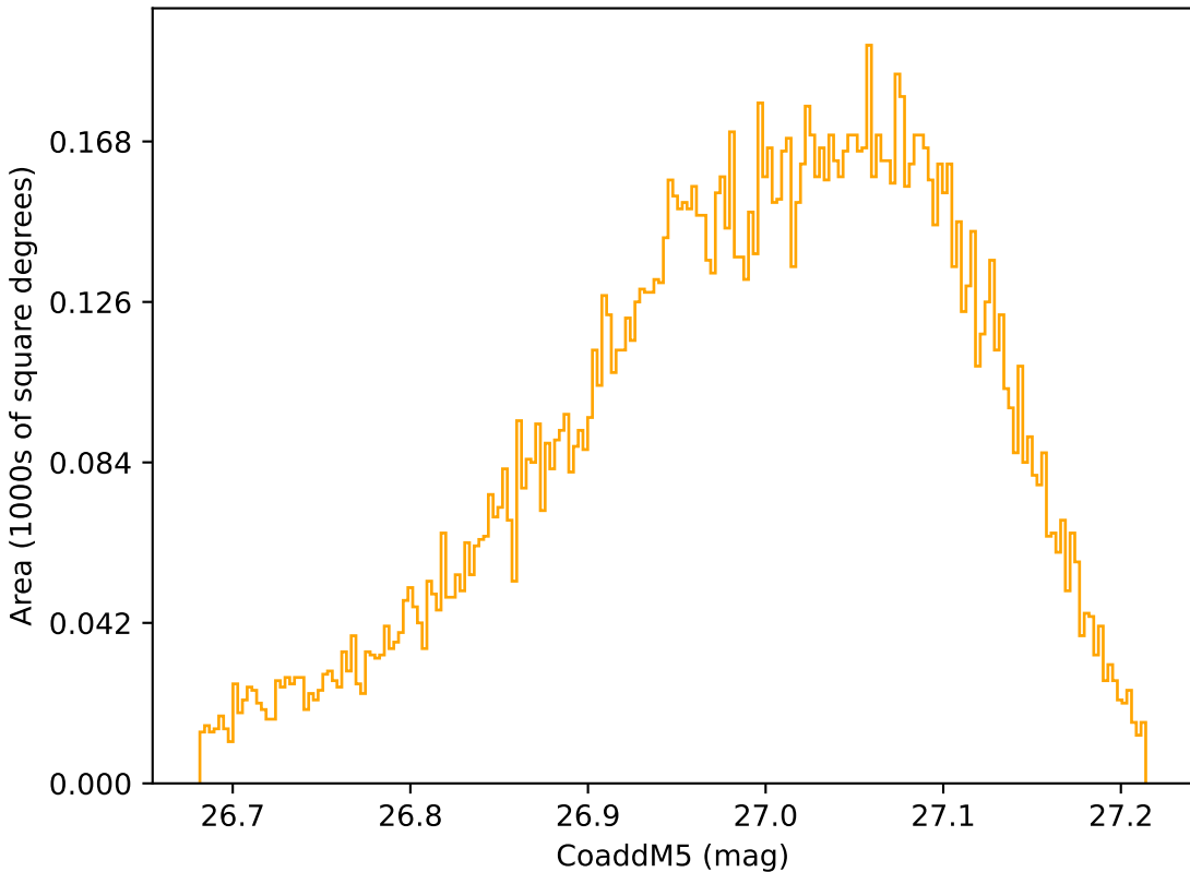
ddf_loaded_half_fl8_v3.4_10yrs WFD r band: CoaddM5
