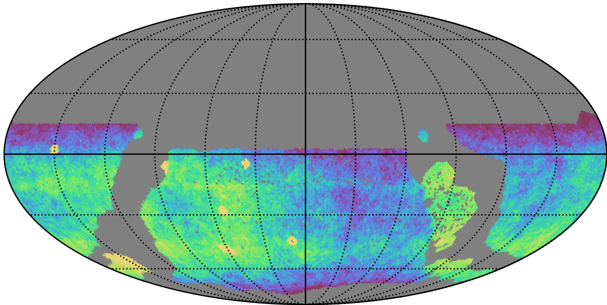
ddf_loaded_half_fl8_v3.4_10yrs WFD g band: CoaddM5
