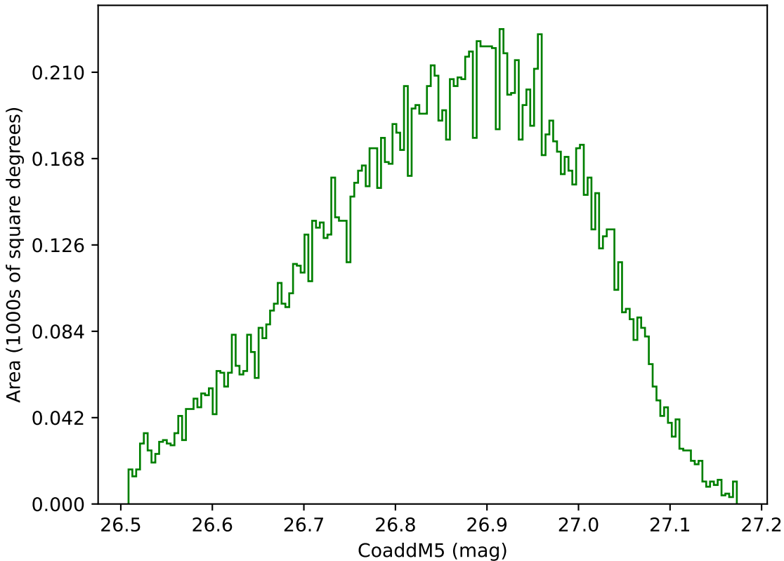
ddf_loaded_half_fl8_v3.4_10yrs WFD g band: CoaddM5
