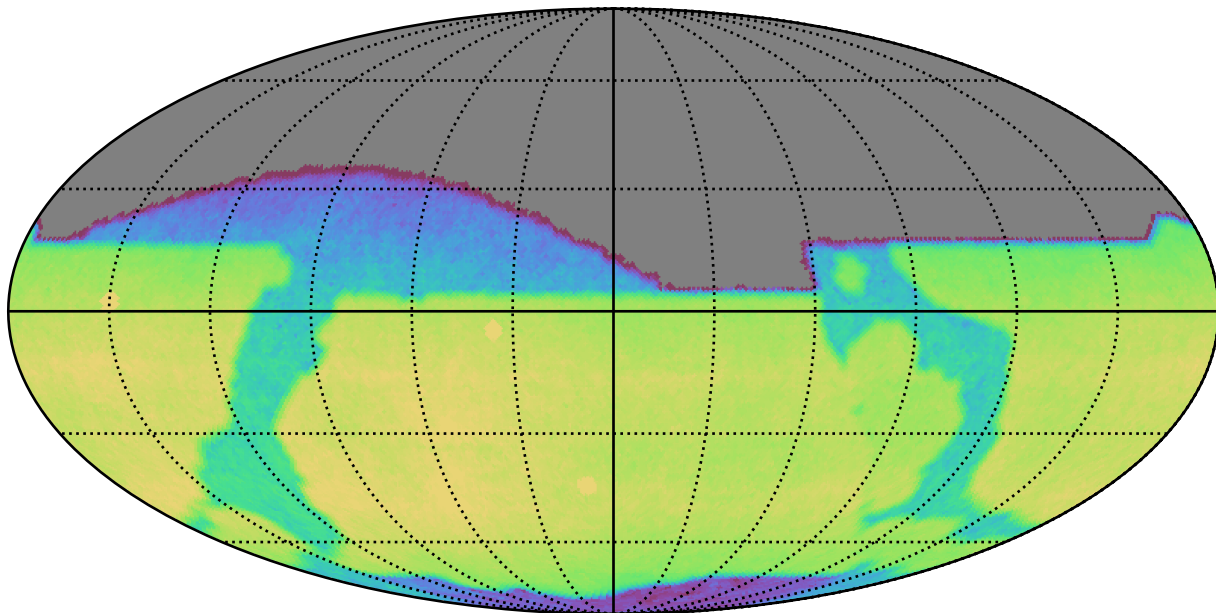
ddf_loaded_half_fl8_v3.4_10yrs All sky z band: CoaddM5
