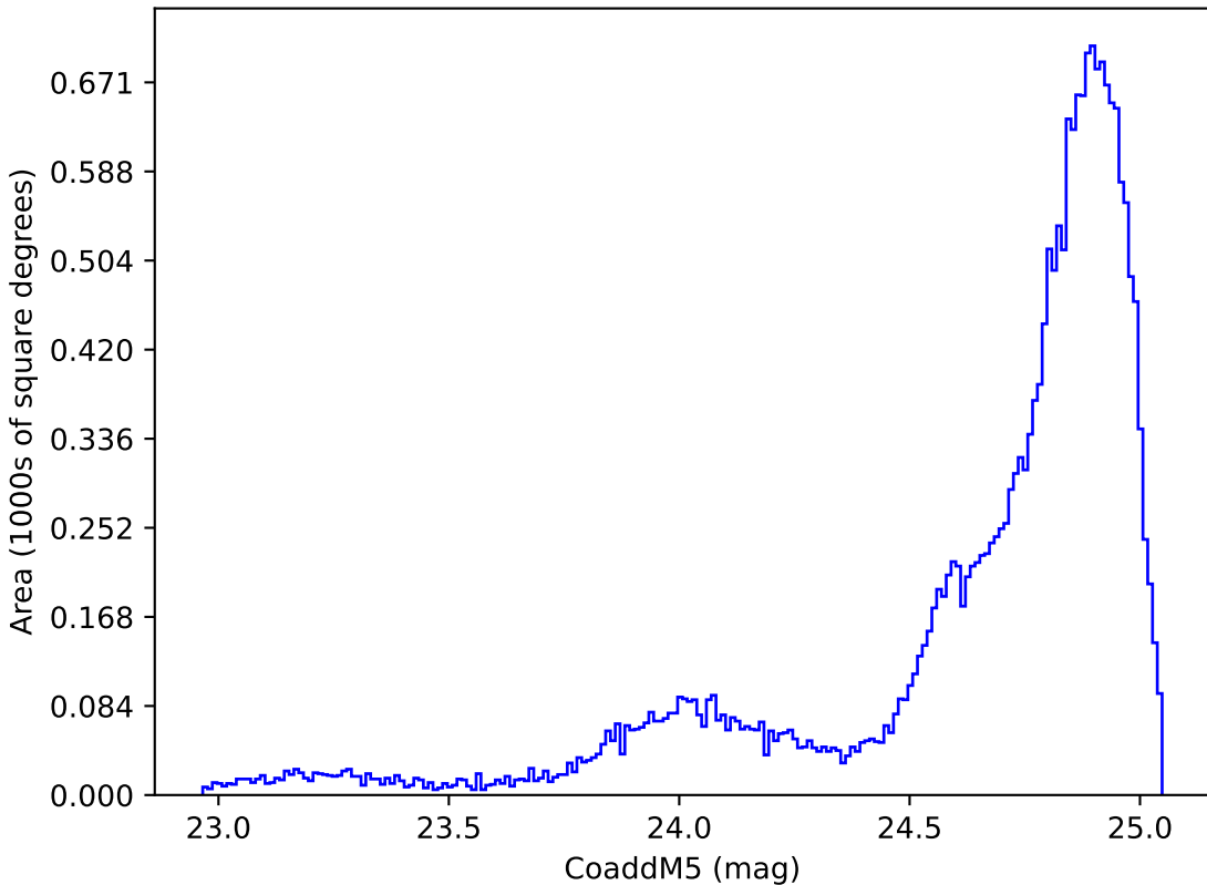
ddf_loaded_half_fl8_v3.4_10yrs All sky y band: CoaddM5
