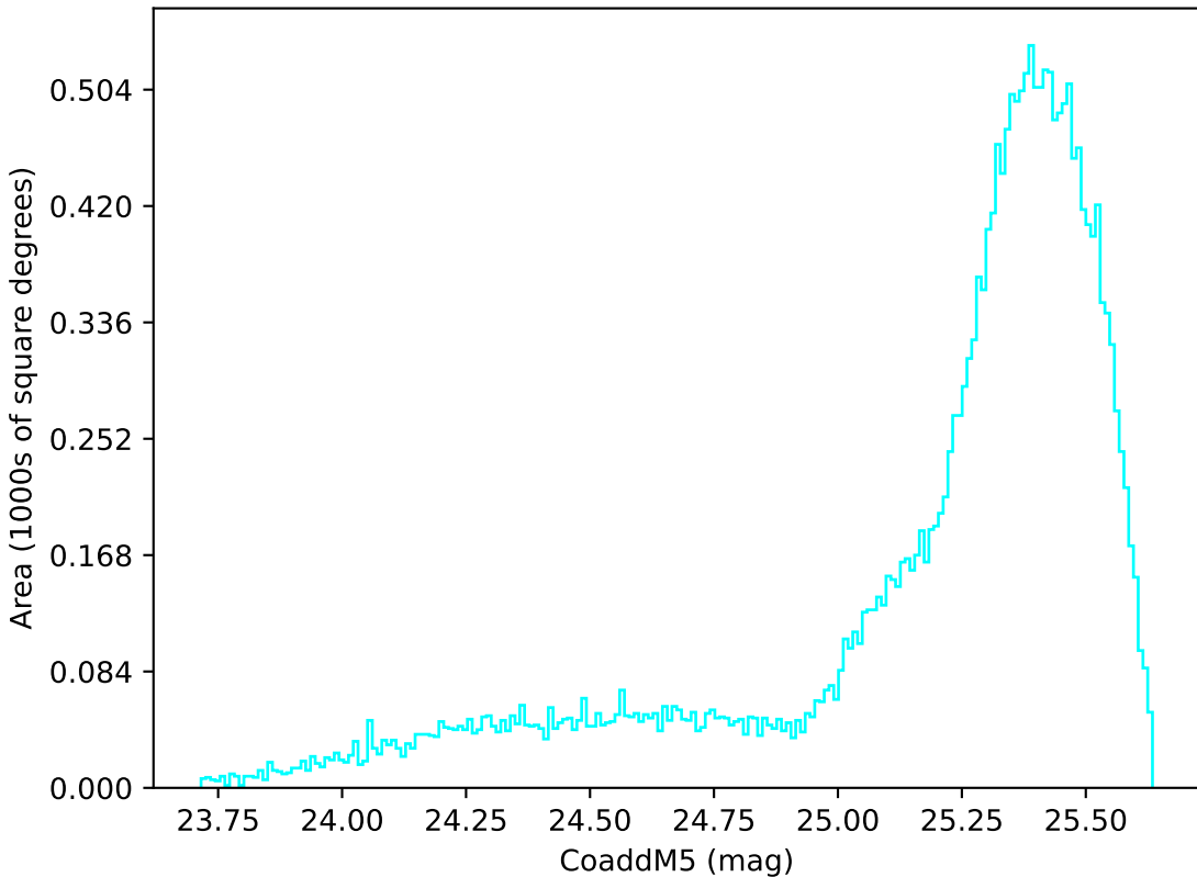
ddf_loaded_half_fl8_v3.4_10yrs All sky u band: CoaddM5
