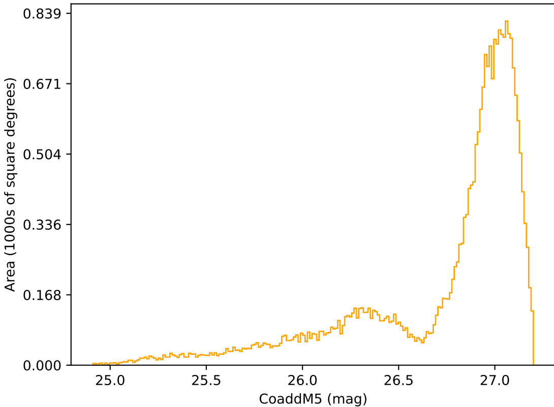
ddf_loaded_half_fl8_v3.4_10yrs All sky r band: CoaddM5
