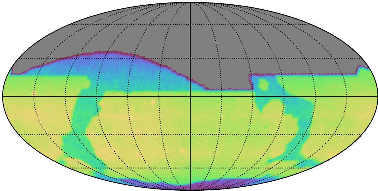
ddf_loaded_half_fl8_v3.4_10yrs All sky i band: CoaddM5
