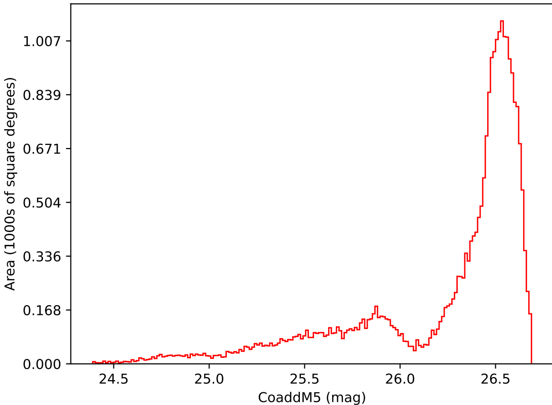
ddf_loaded_half_fl8_v3.4_10yrs All sky i band: CoaddM5
