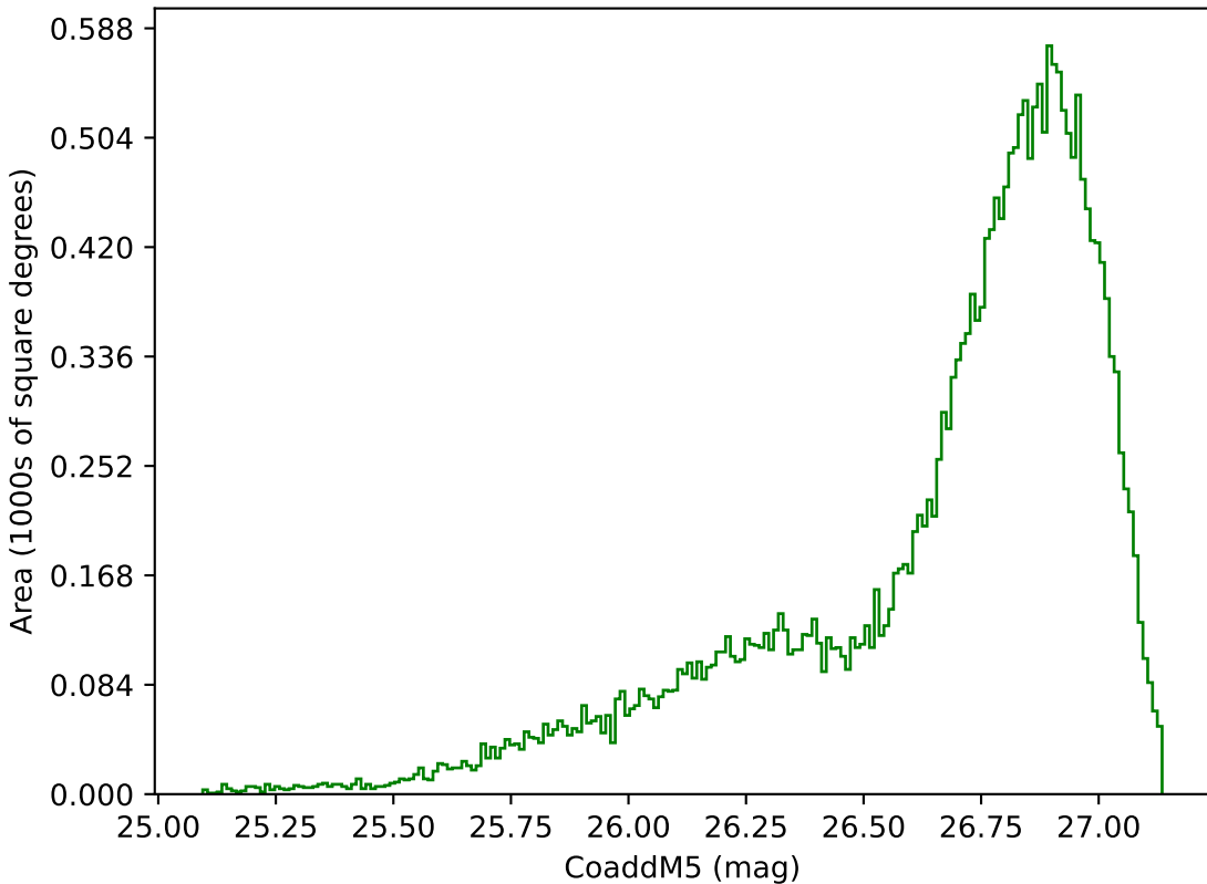
ddf_loaded_half_fl8_v3.4_10yrs All sky g band: CoaddM5
