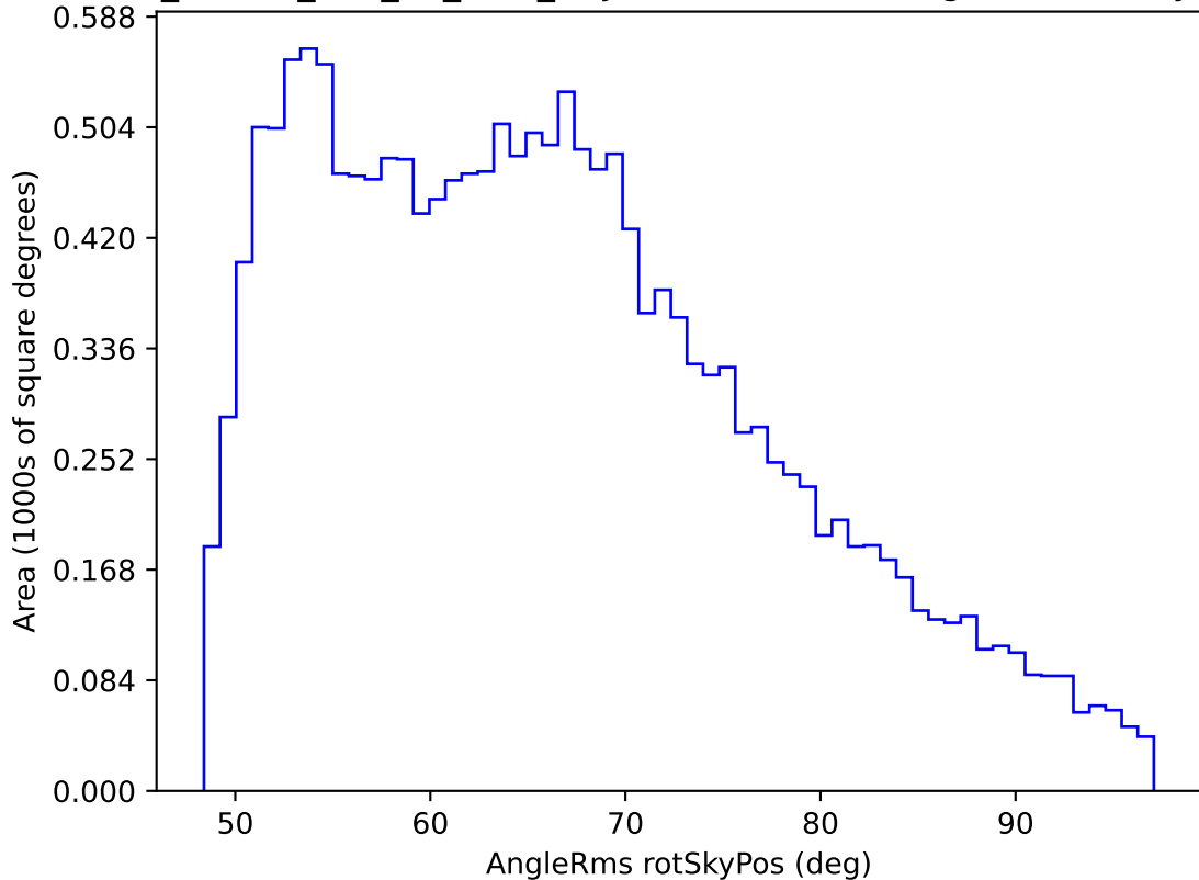
ddf_loaded_half_fl8_v3.4_10yrs WFD r band: AngleRms rotSkyPos
