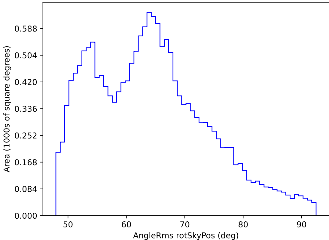
ddf_loaded_half_fl8_v3.4_10yrs WFD i band: AngleRms rotSkyPos
