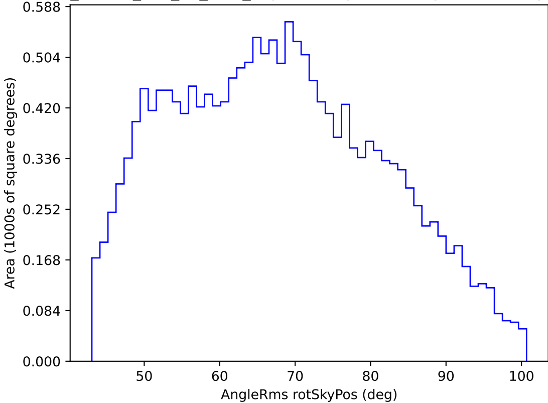
ddf_loaded_half_fl8_v3.4_10yrs WFD g band: AngleRms rotSkyPos
