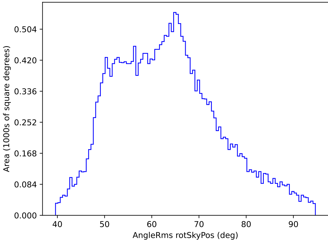
ddf_loaded_half_fl8_v3.4_10yrs All sky z band: AngleRms rotSkyPos
