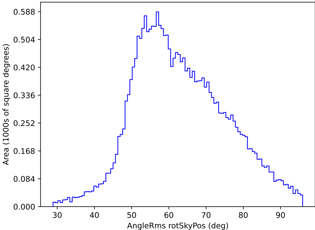
ddf_loaded_half_fl8_v3.4_10yrs All sky u band: AngleRms rotSkyPos
