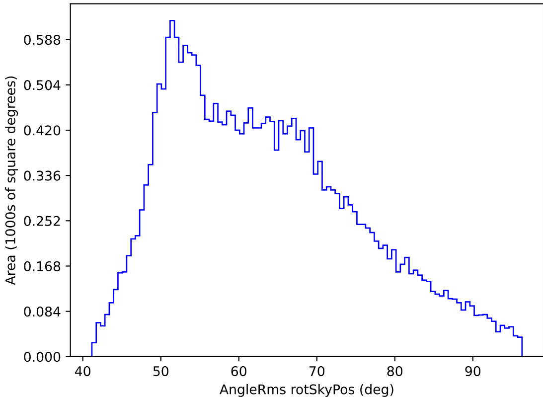
ddf_loaded_half_fl8_v3.4_10yrs All sky r band: AngleRms rotSkyPos
