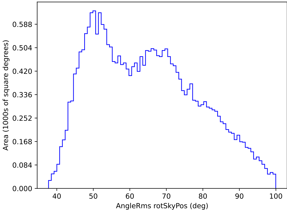
ddf_loaded_half_fl8_v3.4_10yrs All sky g band: AngleRms rotSkyPos
