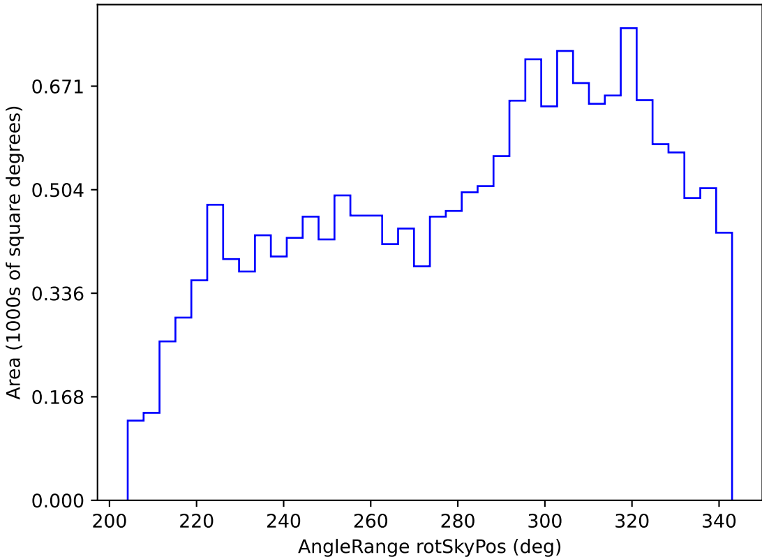
ddf_loaded_half_fl8_v3.4_10yrs WFD r band: AngleRange rotSkyPos
