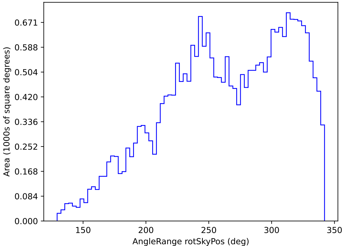
ddf_loaded_half_fl8_v3.4_10yrs All sky z band: AngleRange rotSkyPos
