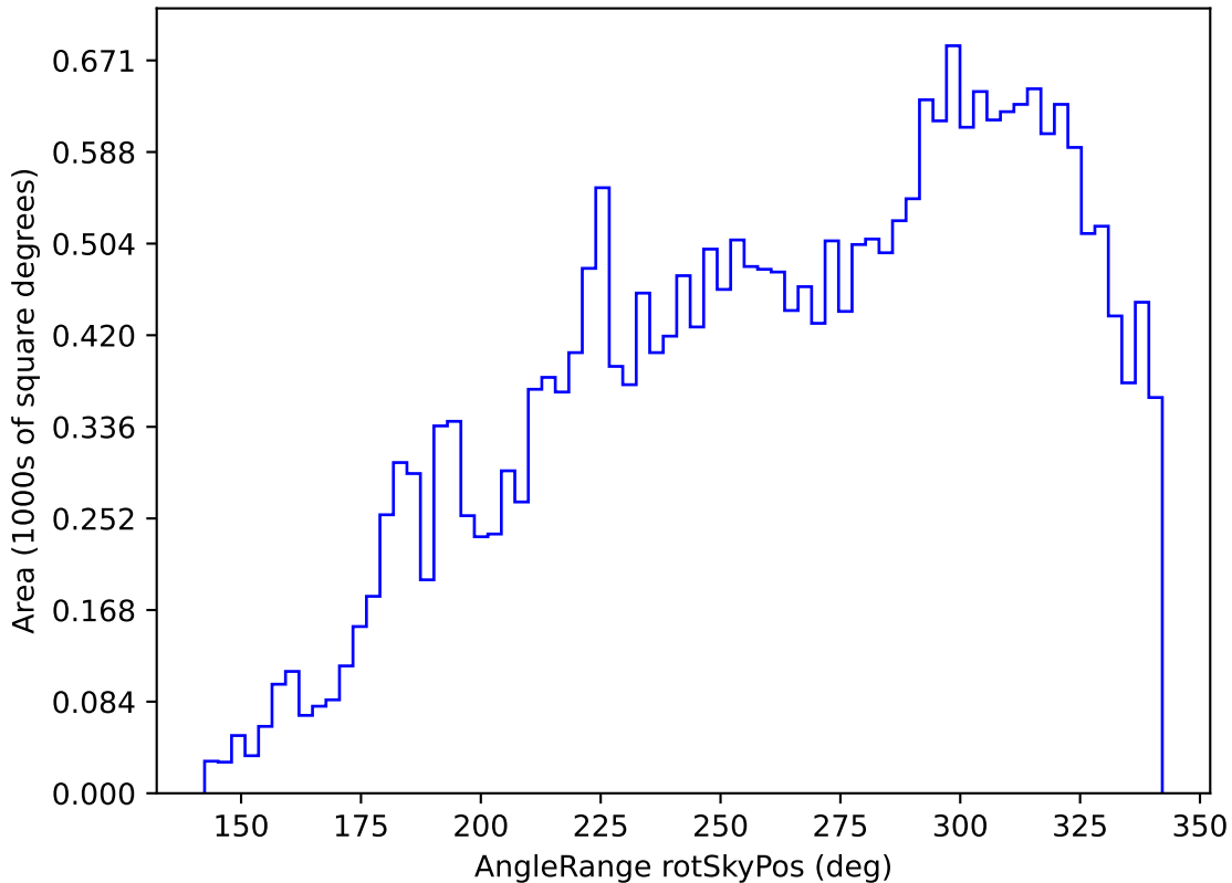
ddf_loaded_half_fl8_v3.4_10yrs All sky r band: AngleRange rotSkyPos
