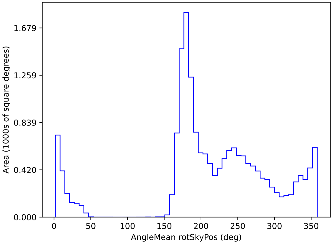
ddf_loaded_half_fl8_v3.4_10yrs WFD z band: AngleMean rotSkyPos
