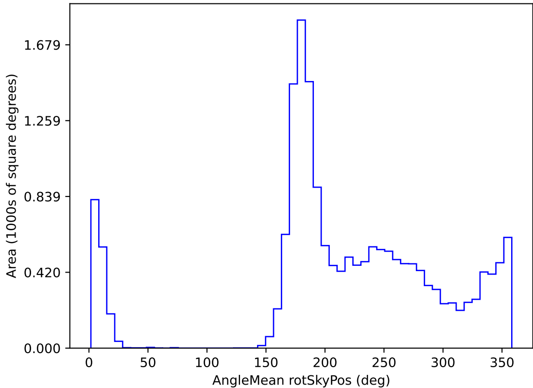
ddf_loaded_half_fl8_v3.4_10yrs WFD y band: AngleMean rotSkyPos
