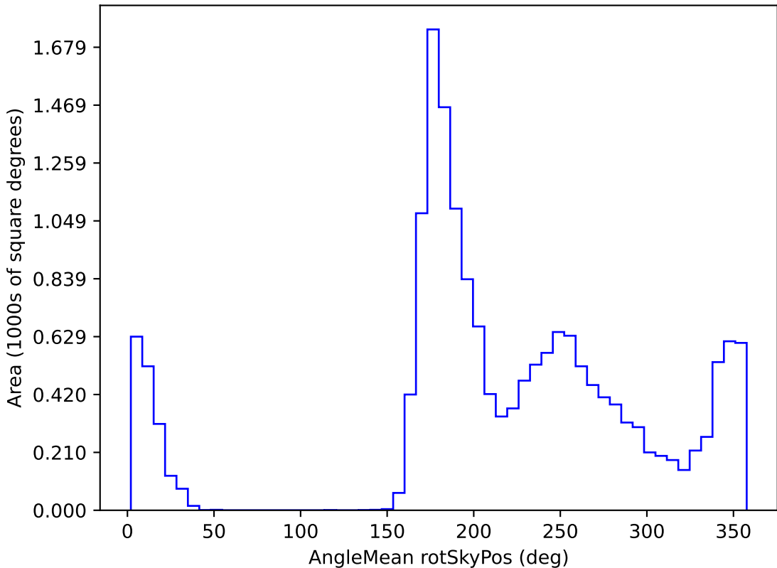
ddf_loaded_half_fl8_v3.4_10yrs WFD i band: AngleMean rotSkyPos
