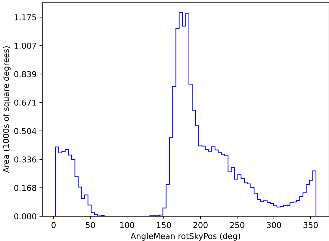
ddf_loaded_half_fl8_v3.4_10yrs WFD g band: AngleMean rotSkyPos
